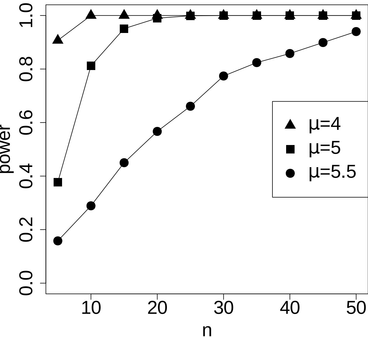
Power Curves with \sigma=1 , H_0: \mu=6
